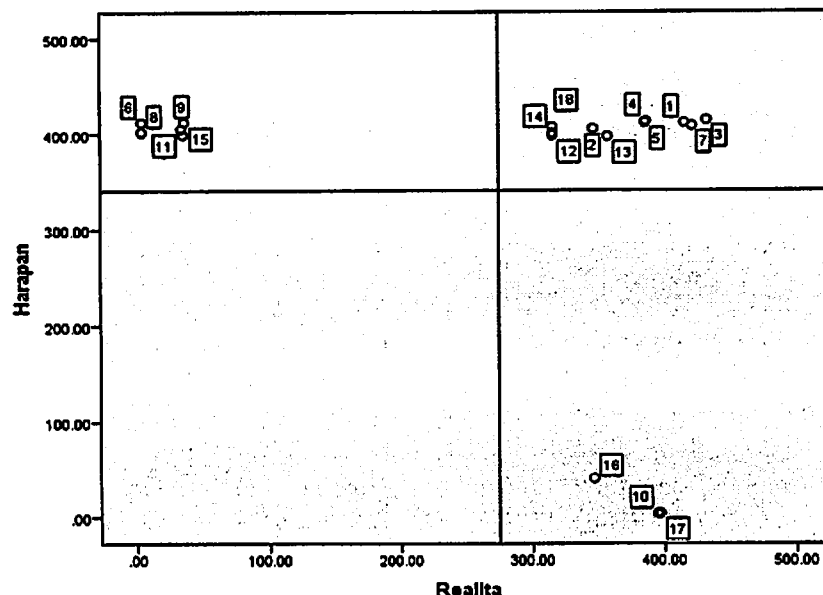
Gambar 2 Diagram Kartesius
